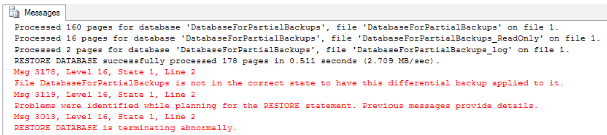
Figure 10-6: Forced failure query results
