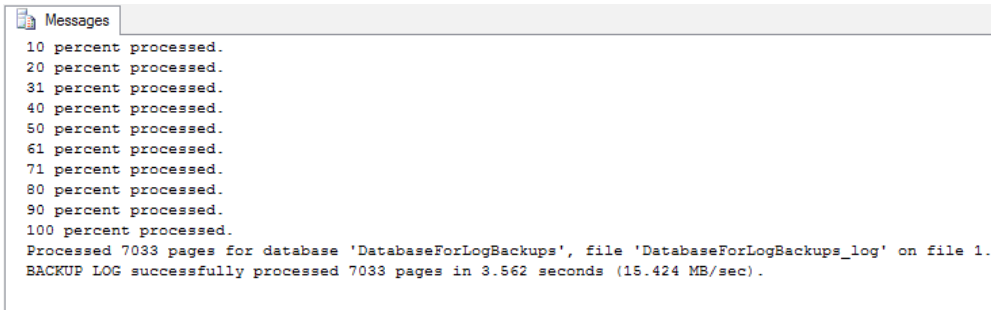
Figure 5-9: Successful transaction log backup message.
