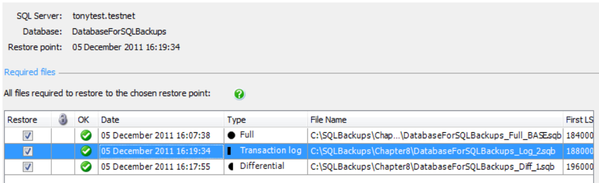
Figure 8-17: Identifying the required files for the restore process.
