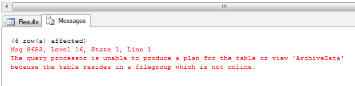
Figure 10-5: Unable to pull information from the archive table.
