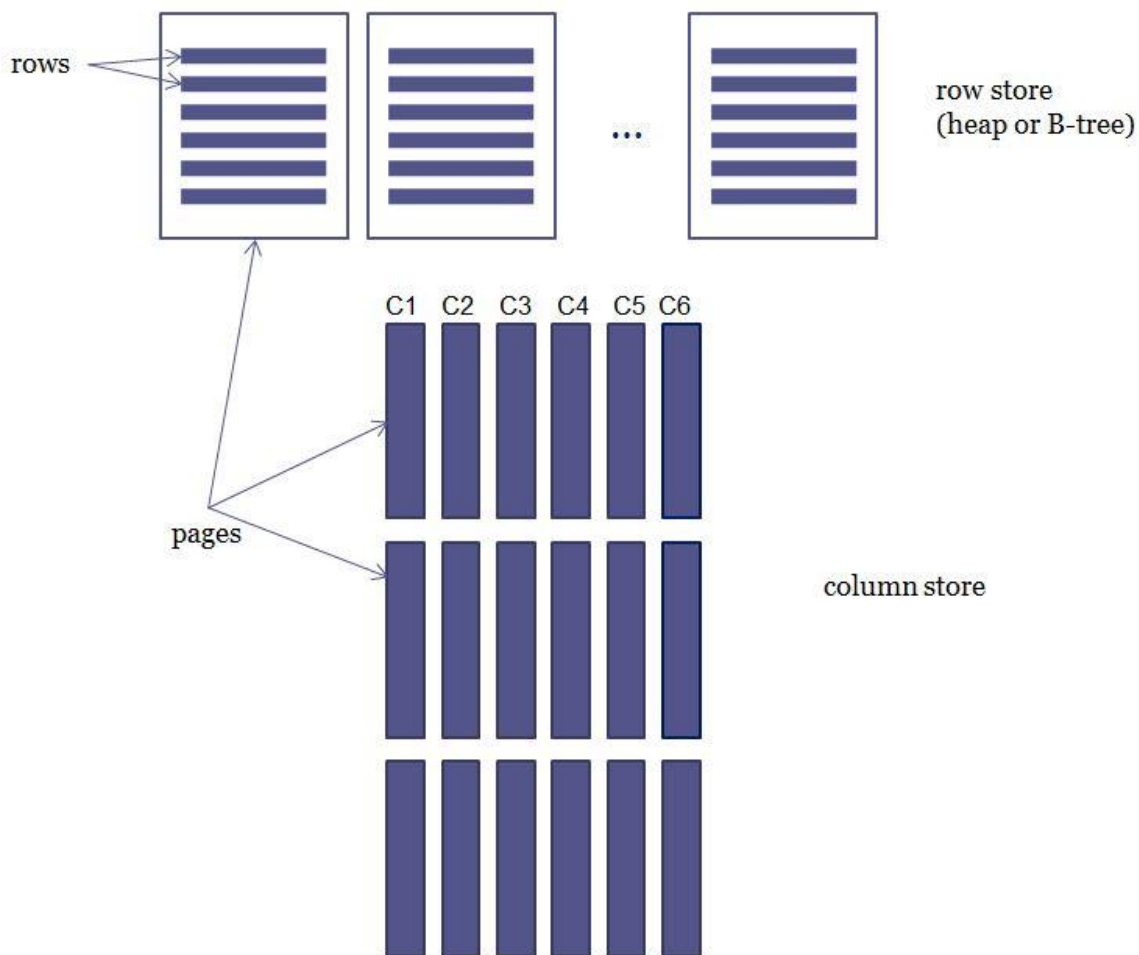
Figure 1: Comparison between row store and column store data layout
